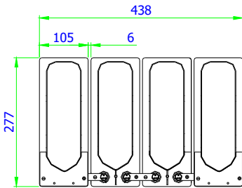
12-50&55 Front Access Battery Height: 223mm
