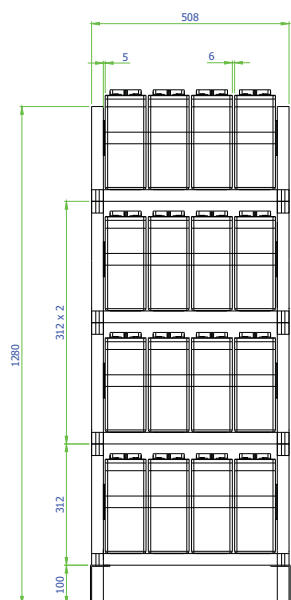
16 x 12V50FA&55FA Rack
