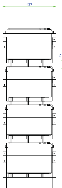
16 x 12V50FA&55FA Rack
