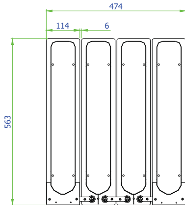
12-70&80 Front Access Battery Height: 182mm
